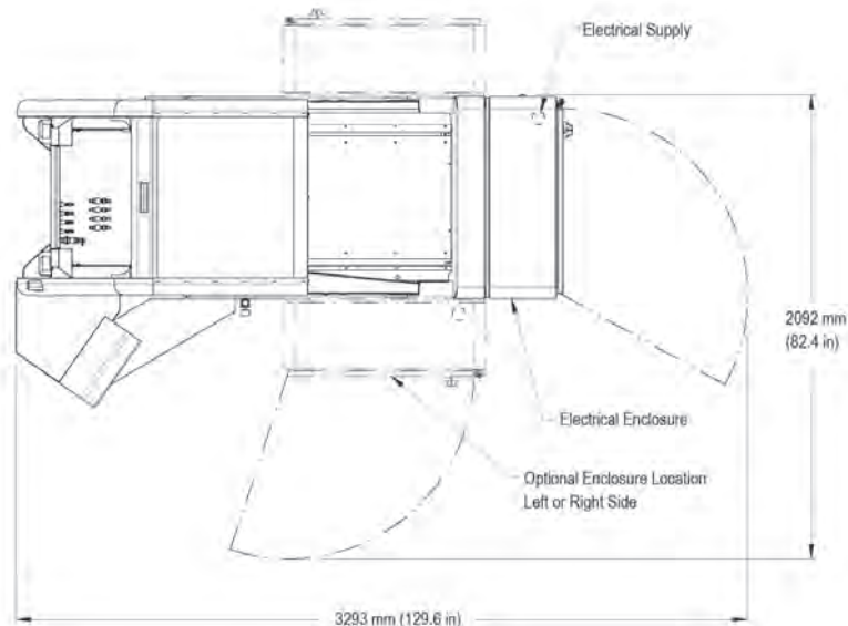
SH-4000 Floor Plan Layout
