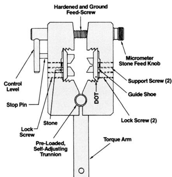
Typical External Honer Body with stone & shoe inserted
